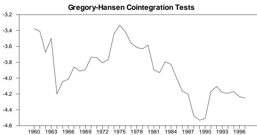
Figure 5: Gregory-Hansen Cointegration Tests
