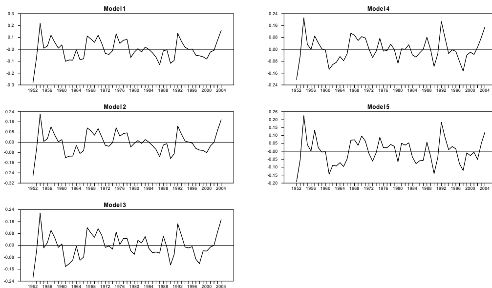
Figure 2: Stationarity of Cointegration Errors
